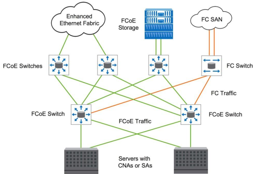
Figure 4) A fully converged network architecture with end-to-end FCoE.
