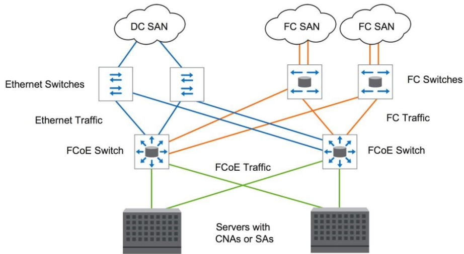
Figure 3) FCoE access switches and CNAs or server adapters (SAs) with FCoE initiators simplify the network topology.
