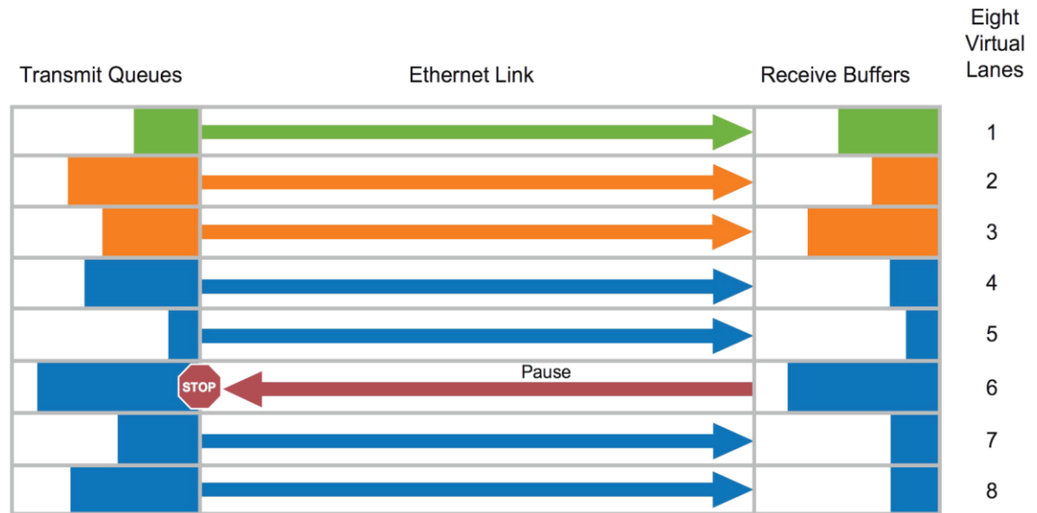
Figure 2) Priority flow control allows up to eight prioritized virtual lanes per Ethernet link.
